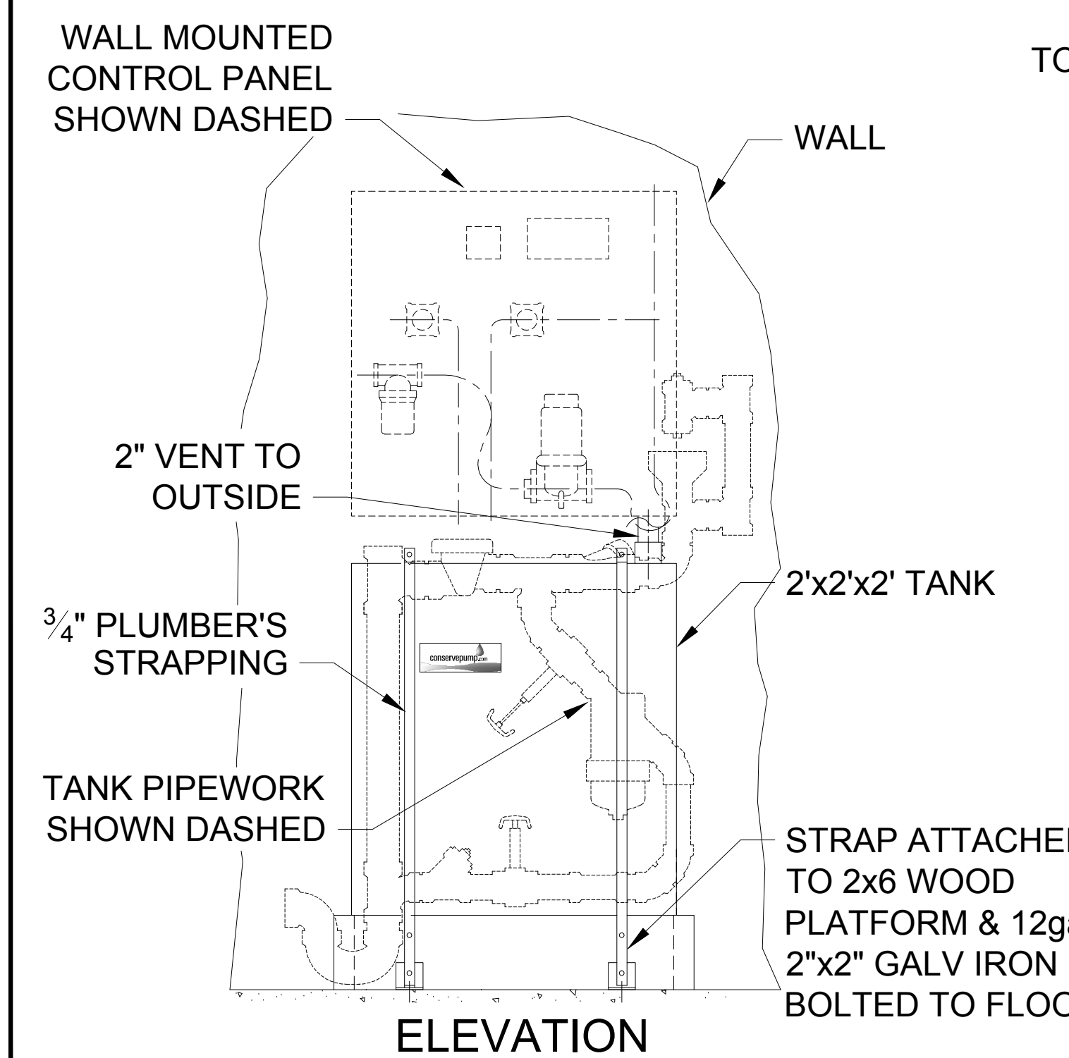
STORAGE TANK INSTALLATION
