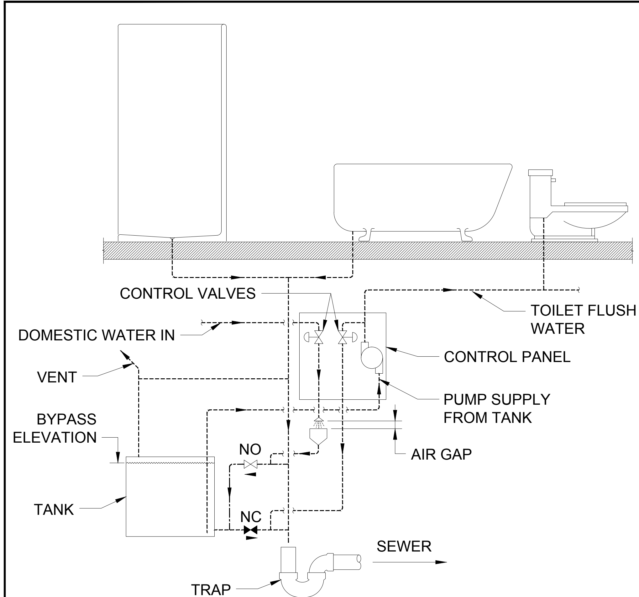
SYSTEM SCHEMATIC DIAGRAM
