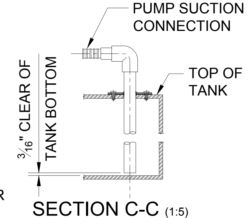
STORAGE TANK INSTALLATION
